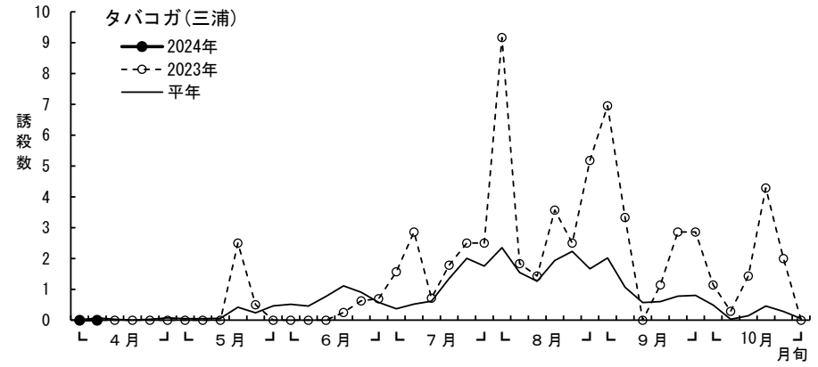
(5)タバコガ
