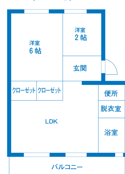
1LDKU [吾妻] (1LDKU)
