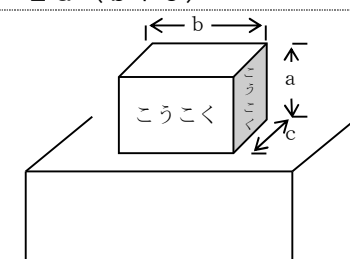
例 2 S = 2 a (b + c)
