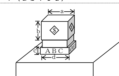
例 6 S = 4 (a b + c d)
